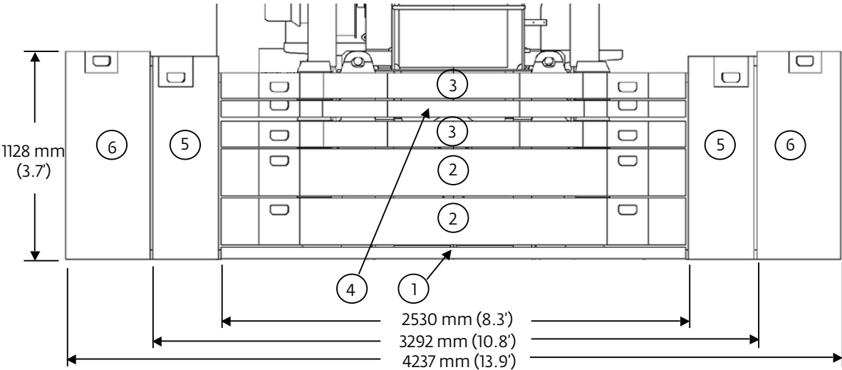
Counterweight configurations
